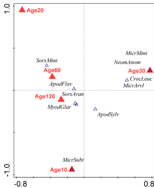
Figure 4. Partial canonical correspondence analysis biplot with the study month as a covariable showing the change in small mammal assemblages in relation to different forest successional stages. ApodFlav , Apodemus flavicollis ; ApodSylv , Apodemus sylvaticus ; MicrSubt , Microtus subterraneus ; MicrArvl , Microtus arvalis ; MicrMint , Micromys minutus ; MyodGlar , Clethrionomys glareolus ; CrocLeuc , Crocidura leucodon ; NeomAnom , Neomys anomalus ; SorxAran , Sorex araneus ; SorxMint , Sorex minutus .
